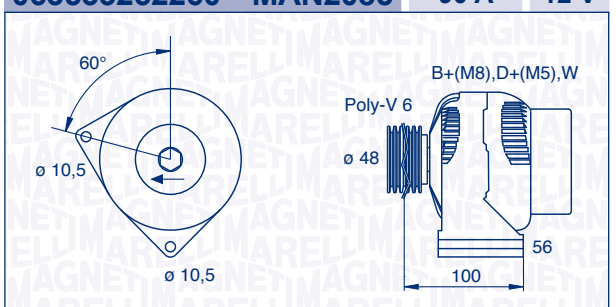
063533252260 – MAN2085 90 A 12 V
