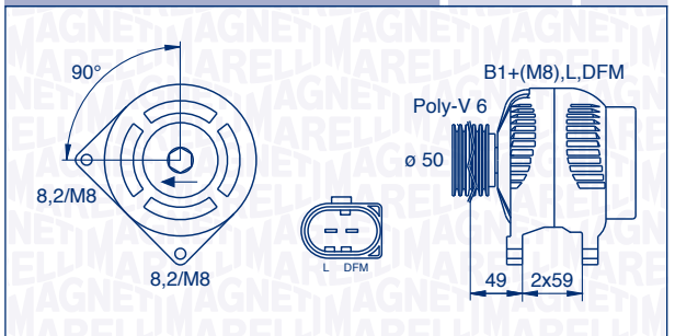
063533250130 – MAN2038 90 A 12 V
