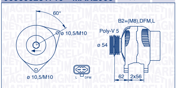
063533251710 – MAN2066 100 A 12 V
