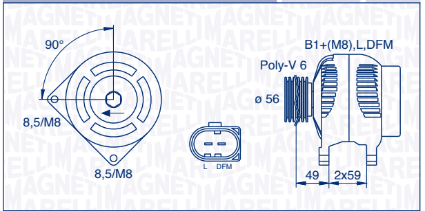
063533250010 – MAN2037 90 A 12 V
